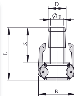
QCC C-Coupler Hose Shank
